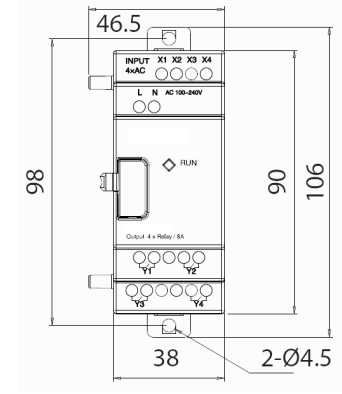
Expansion Modules
